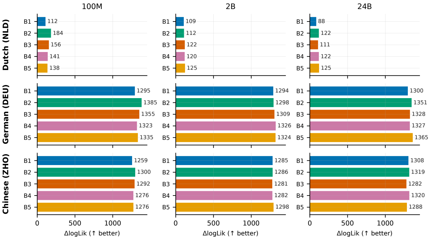
F9 — Curriculum effect on cognitive fit, per L1 x training scale
